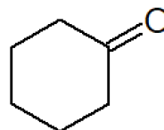
cyclohexanone
